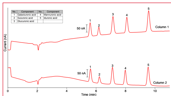
Fig. 6. Chromatograms of each column obtained from a 2.5 \mu L injection of 10 \mu M standard mix containing uronic acids in DI water.
