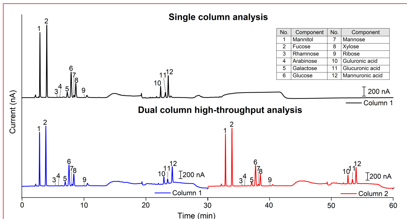
Fig. 1. Example chromatograms of 2.5 µL injections of 20× diluted acid-hydrolyzed seaweed sample on (top) single column analysis on column 1, and (bottom) dual column high-throughput analysis on column 1 (blue), and on column 2 (red). Approximately 2× faster analysis time was achieved with the dual column high-throughput analysis.
