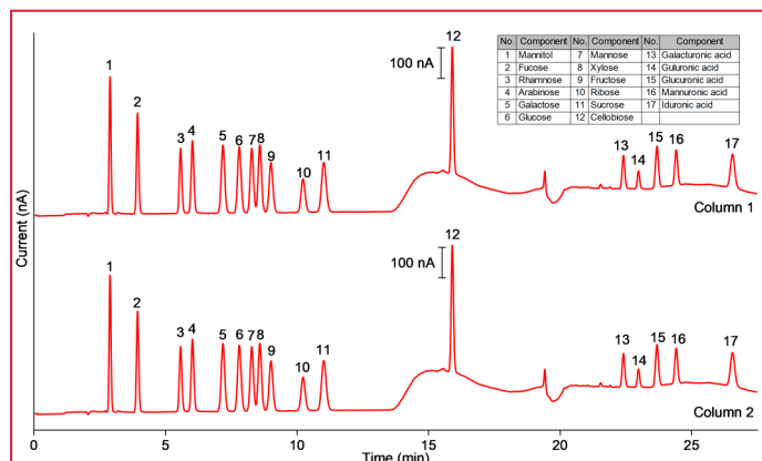
Fig. 3. Example chromatograms of each column injecting 2.5 µL of a 10 µM standard mix containing neutral sugars and uronic acids in DI water. Separation and detection was achieved using the HPAEC-PAD conditions and gradient program shown in Table 1 and 2, respectively.
