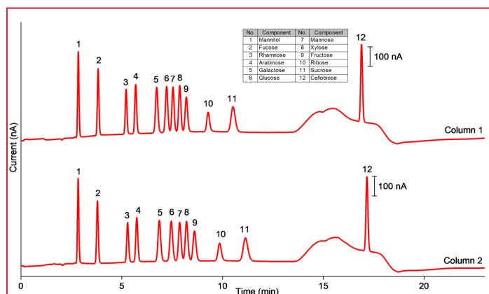
Fig. 5. Chromatograms of each column obtained from a 2.5 \mu L injection of 10 \mu M standard mix containing neutral sugars in DI water.
