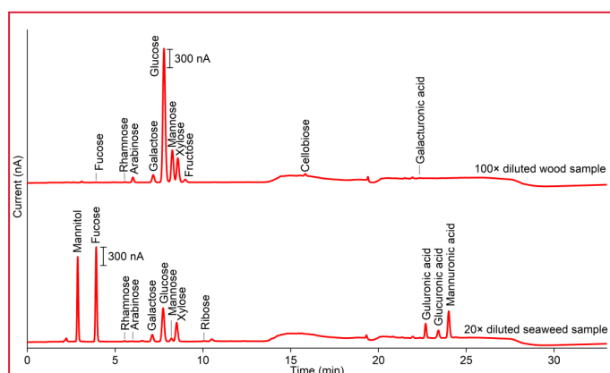
Fig. 4. Overlay of chromatograms obtained from 2.5 µL injections of the wood (100-fold diluted, top) and the seaweed hydrolysate (20-fold diluted, bottom).
